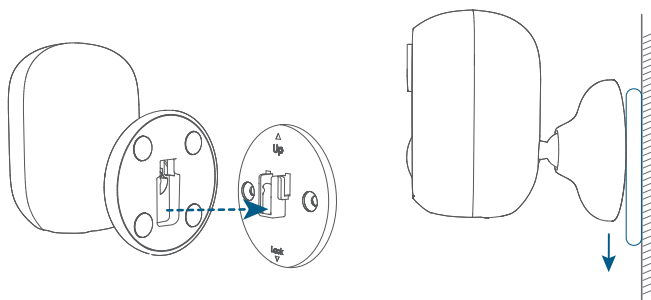
⑤ Slide the Camera onto the Mounting Base
